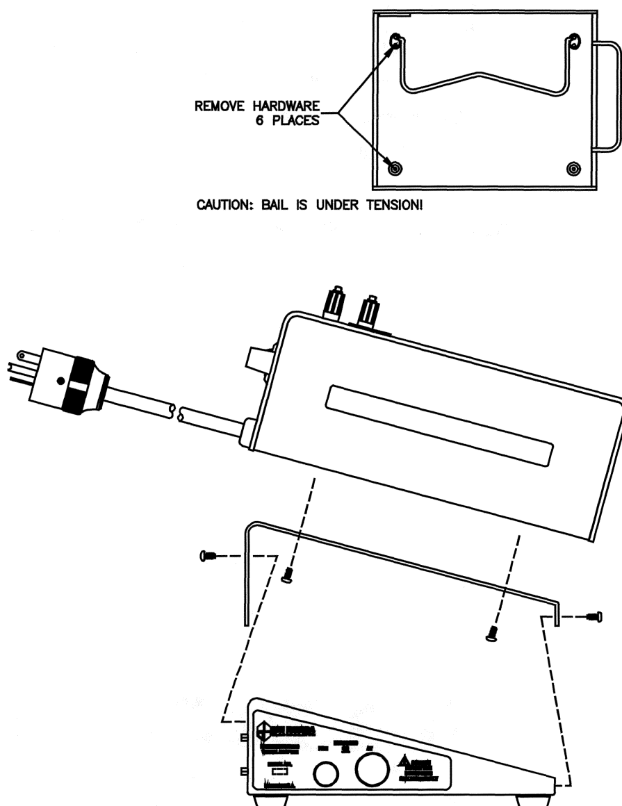
Figure 13-1. Wedge Installation
